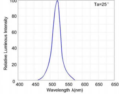
Wavelength Characteristics
