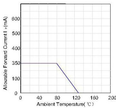
Allowable Forward Current - Ta
