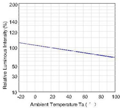
Relative Luminous Intensity - Ta
