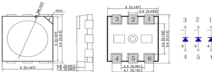
Packing for single LED
