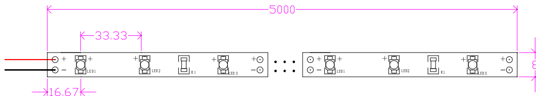
Packing for single LED
