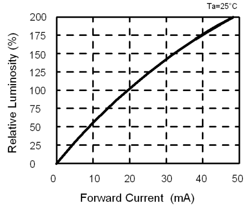
FIG. 2 Relative Luminosity Vs. Forward Current
