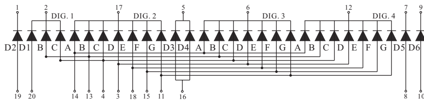
CODE L
